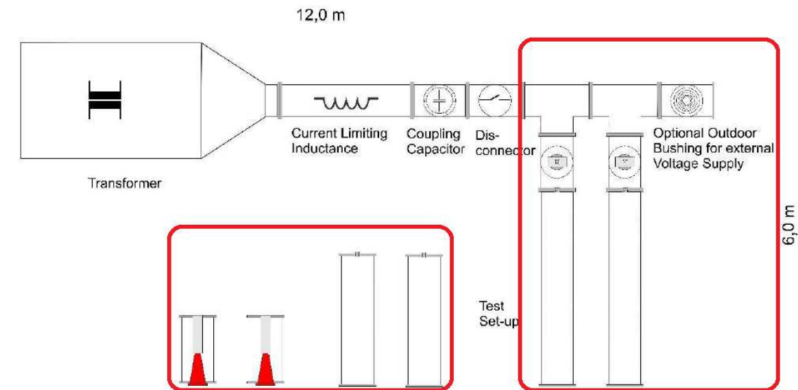
Figure 1. Layout of the complete Test Equipment
